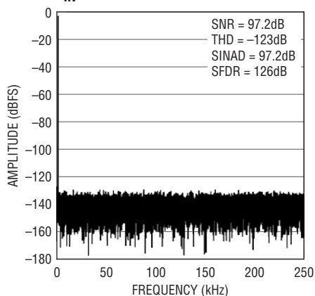
32k Point FFT f_S = 500\text{kps} , f_{IN} = 2\text{kHz}
